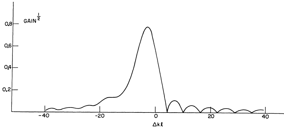
FIG. 5. Variation of the total gain with phase matching for relative crystal length u=5.55 , degeneracy parameter \mu=0.5 , and relative focusing of signal to pump \nu=1.0 .
