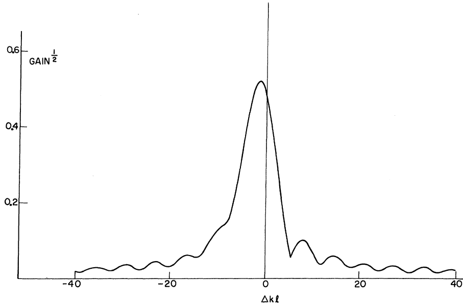
FIG. 4. Variation of the total gain with phase matching for relative crystal length u=0.5 , degeneracy parameter \mu=0.5 , and relative focusing of signal to pump \nu=1.0 .
